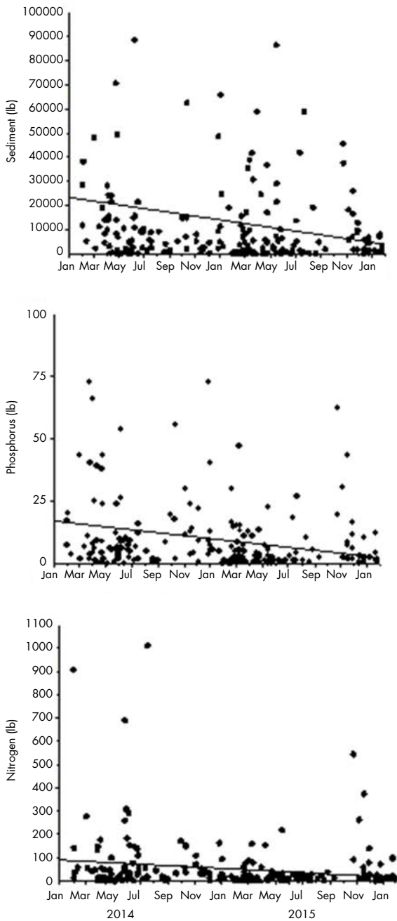
Figure 3. Sediment and nutrient loads leaving fields and running off into TWR systems annually (monitored for 2 years). Six TWR systems were monitored. The systems were within watersheds ranging from 141 to 385 acres and were all tilled land (except for turn rows). Solid lines represent the trend over the 2-year monitoring period.
