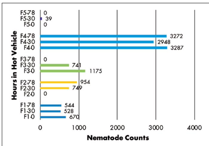
Figure 3. Root-Knot: Transportation
