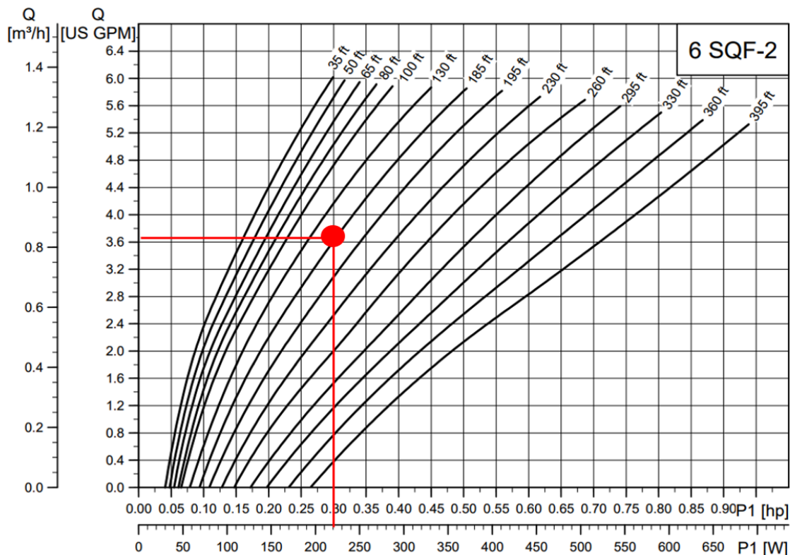
Figure 1. Example pump curve for Grundfos SQFlex helical solar water pump model 6 SQF-2.
