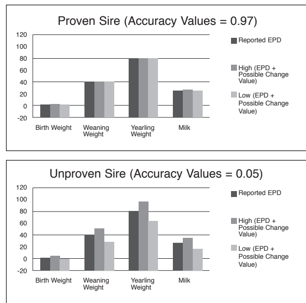
Figure 1. Accuracy and possible EPD change example of expected progeny differences for two bulls.
